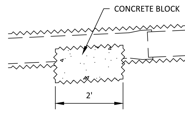
AERIAL SANITARY SEWER STABILIZER BLOCK NOT TO SCALE
