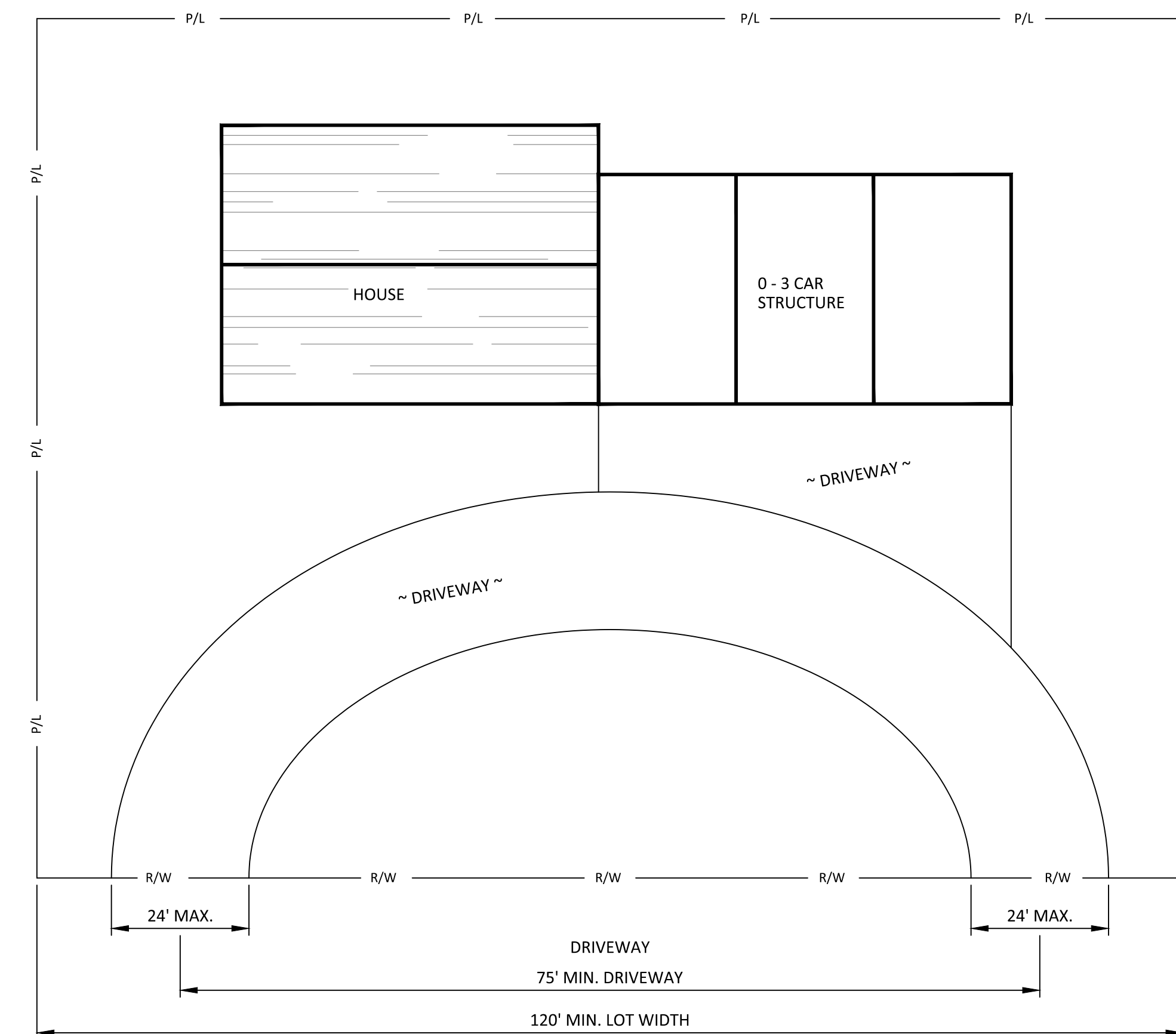
CIRCLE DRIVE (NOT TO SCALE)
