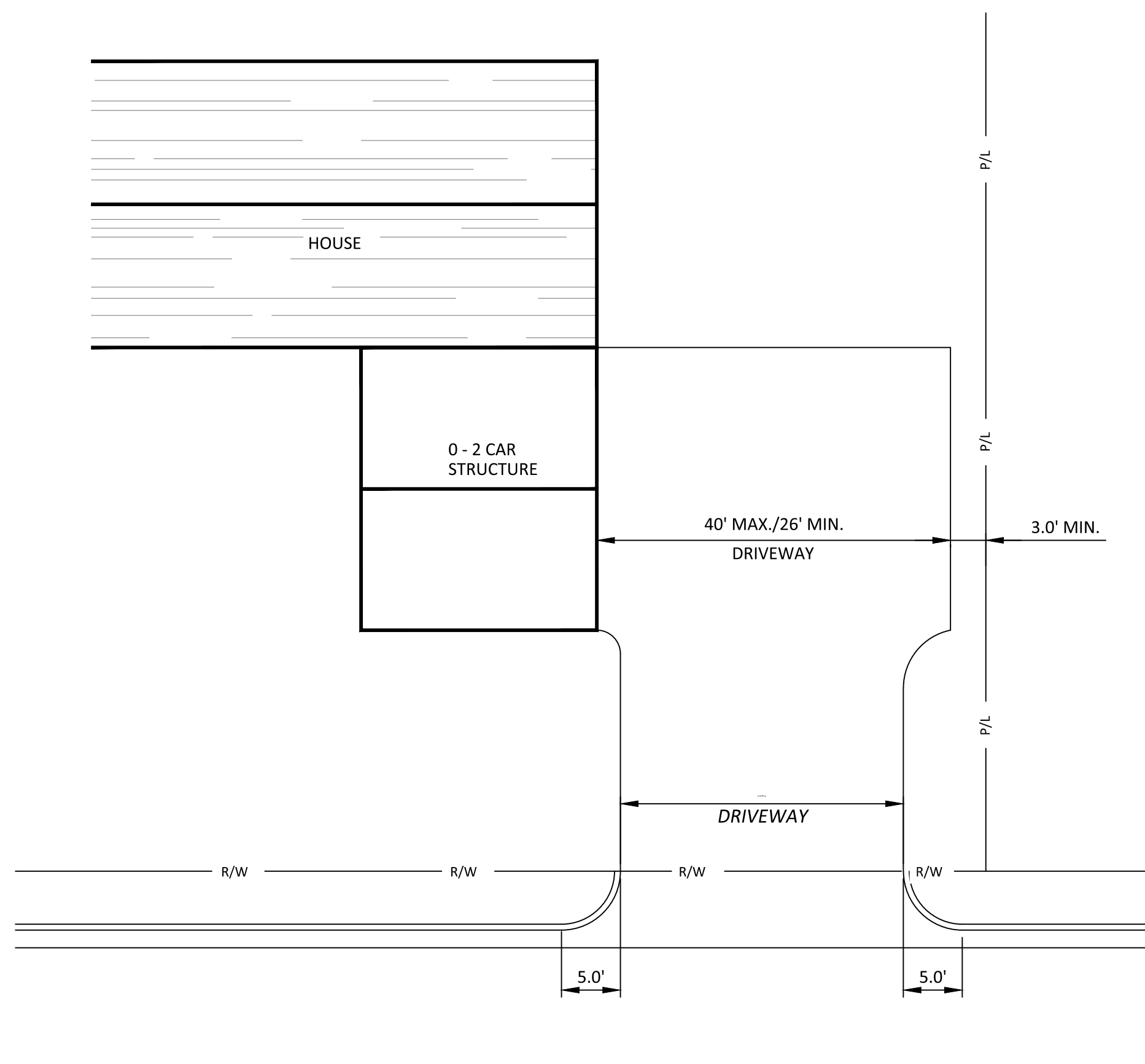
SIDE-LOADED GARAGE (NOT TO SCALE)
