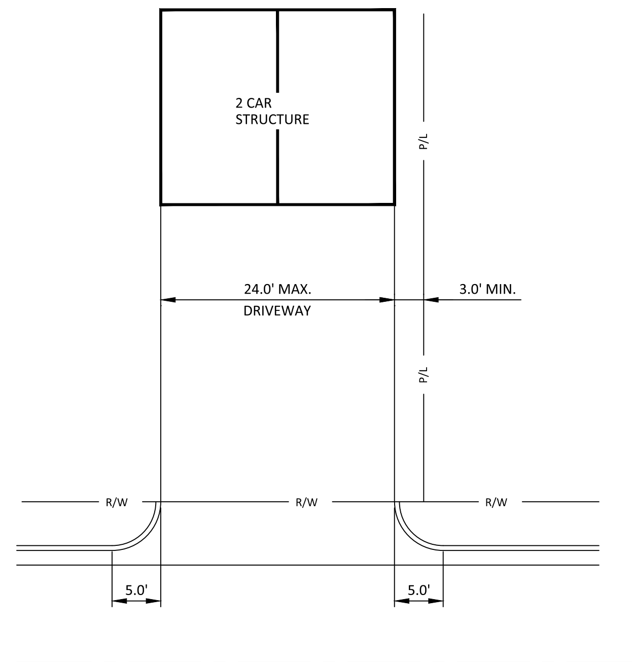
0 - 2 CAR STRUCTURE (NOT TO SCALE)
