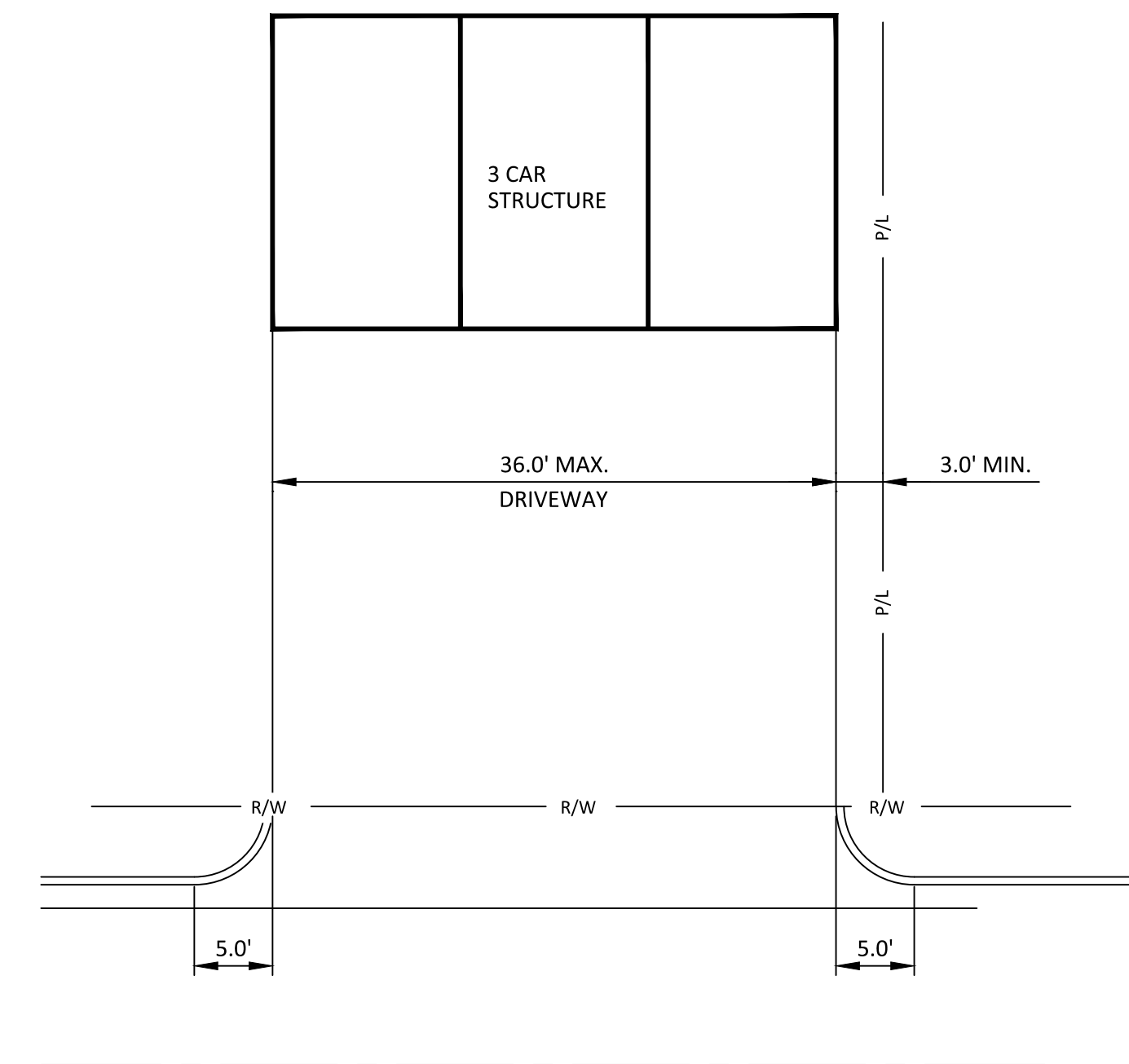
3 CAR COVERED STRUCTURE (NOT TO SCALE)
