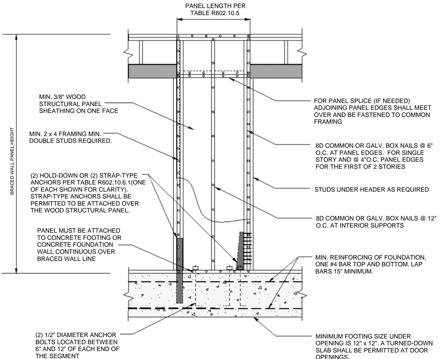
Figure R602.10.6.1 – ALTERNATE BRACED WALL PANEL
